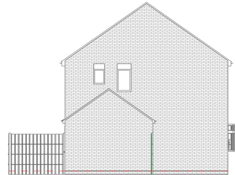
Proposed South East Elevation
